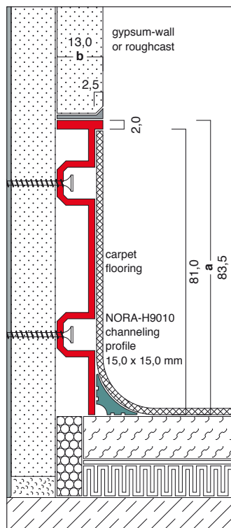
C12/U with NORA-channeling-profile
