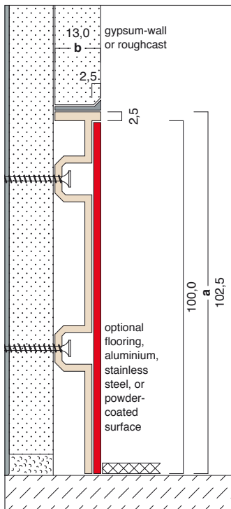
C8/U-A 102,5 x 13,0 mm
