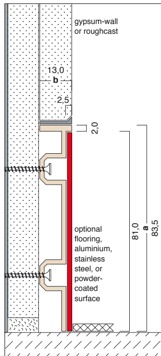
C12/U-A 82,5 x 13,0 mm
