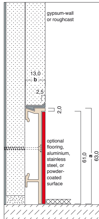
C22-A 63,0 x 13,0 mm
