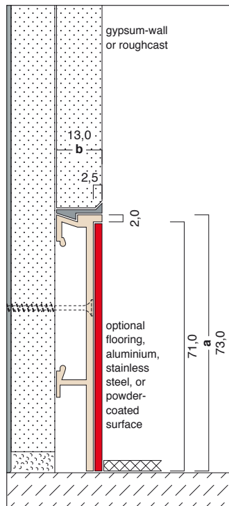
C23-A 73,0 x 13,0 mm
