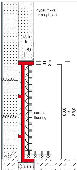
A1 85,0 x 13,0 mm
