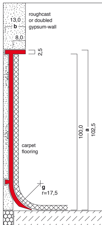
E4 100,0 x 13,0 mm
